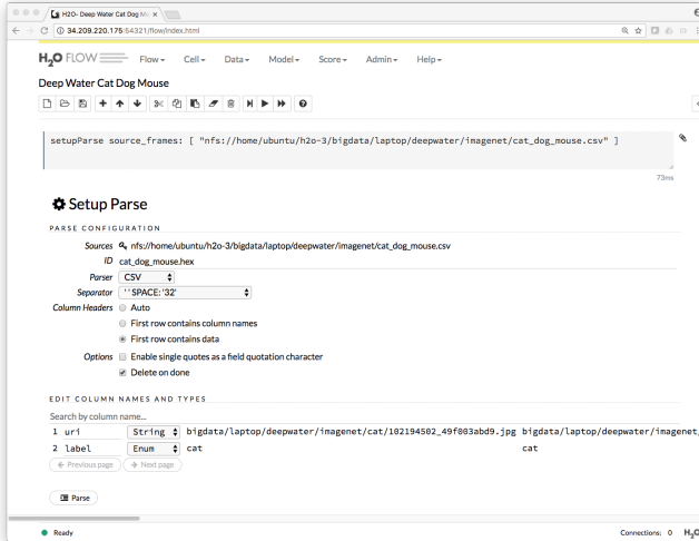
Figure 2: Parse data
