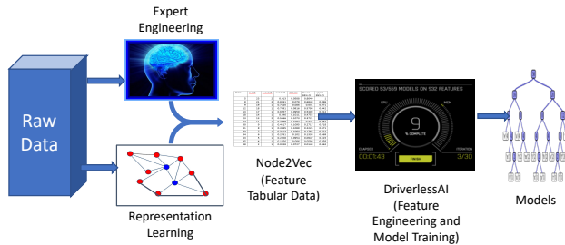
Figure 1: Modelling Pipeline
